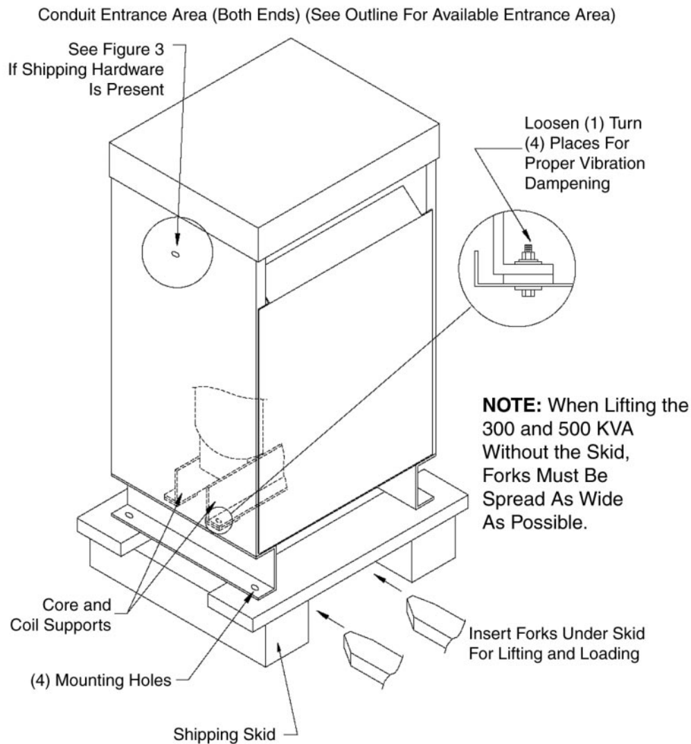
Figure 2 - Typical Assembly for NEMA 2 Enclosures
