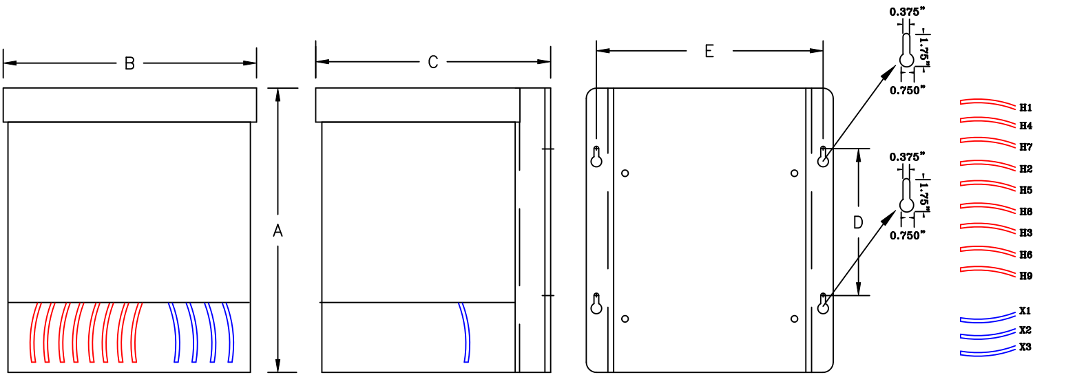
FRONT VIEW
