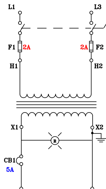
CIRCUIT VIEW
