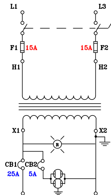
CIRCUIT VIEW
