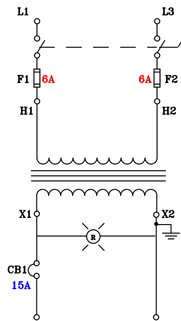
CIRCUIT VIEW
