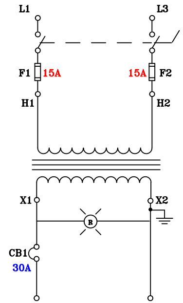
CIRCUIT VIEW
