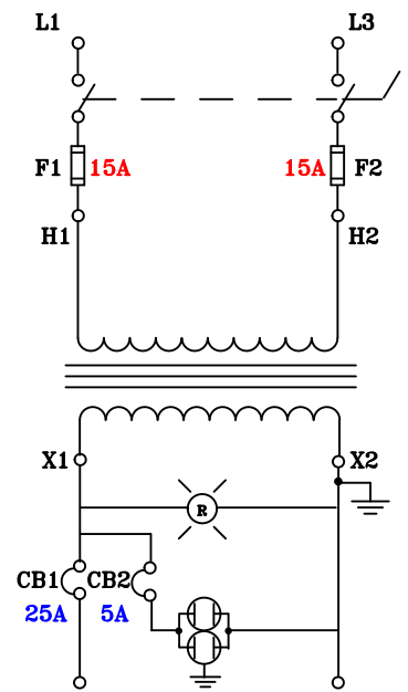
CIRCUIT VIEW
