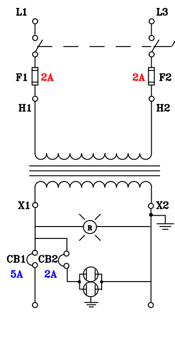
CIRCUIT VIEW
