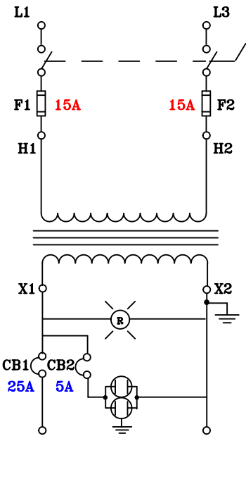
CIRCUIT VIEW
