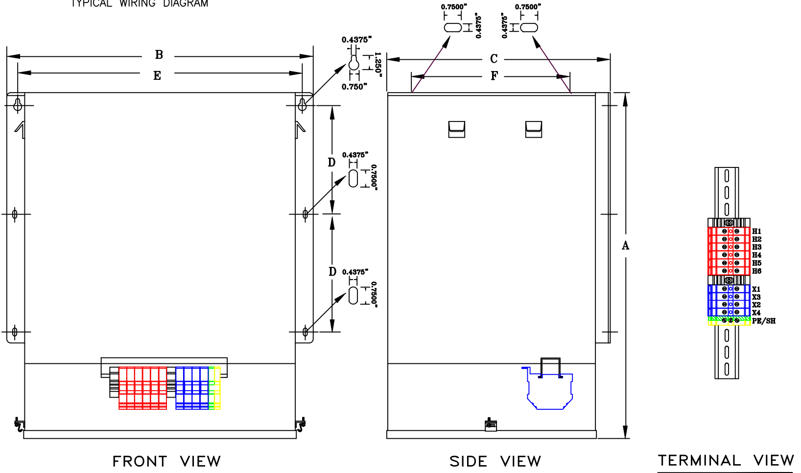
TYPICAL WIRING DIAGRAM
